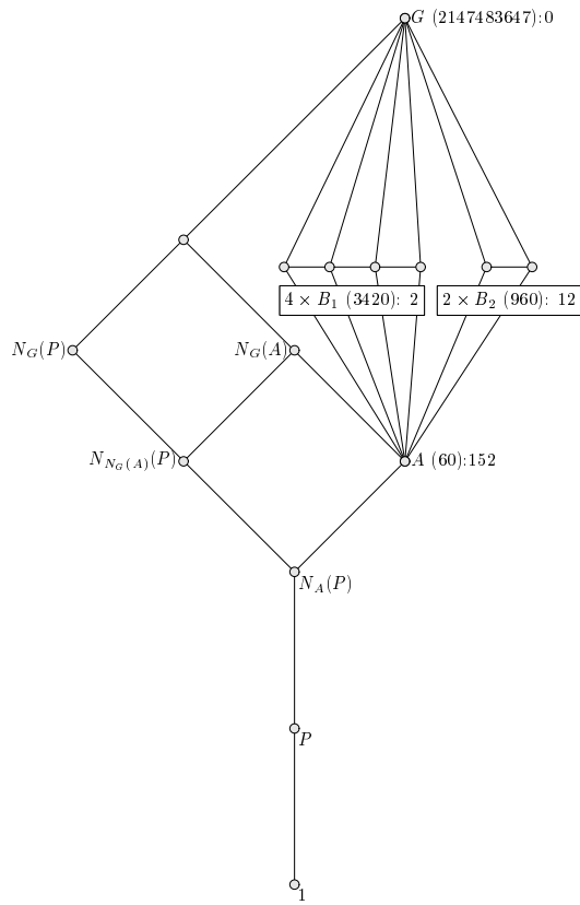
Figure 4: Partial Subgroup Lattice of S_{20} Relevant for Certain SQS(20)
