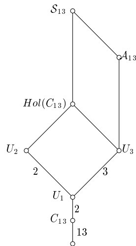
Figure 2: Partial Subgroup Lattice of S_{13} Relevant for 2-(13, 5, 72). The Numbers Between two Subgroups Denote the Indices.
