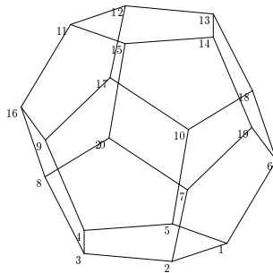
Figure 3: Labeled Dodecahedron
